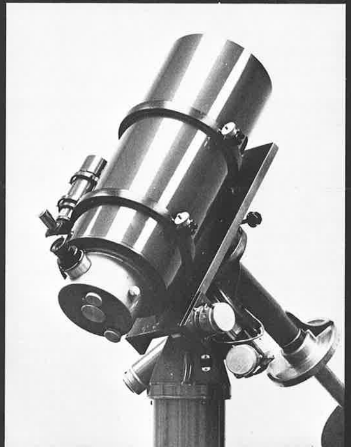
QUANTUM EIGHT BARREL ASSEMBLY ON GERMAN EQUATORIAL MOUNT.
